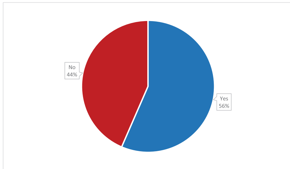
Figure 3.5: Issue resolving
